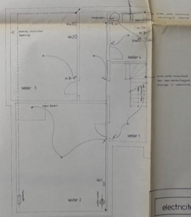
kelderplan
